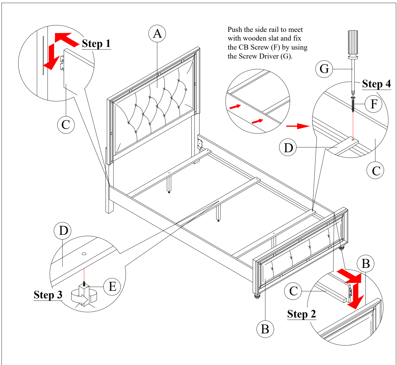
COMPLETED FULL BED ASSEMBLY
